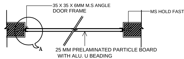
SECTION AT X'-X' N.T.S.
